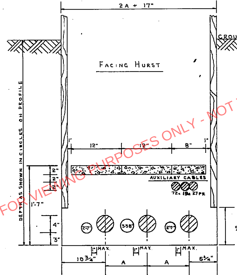
C.S.A. EVEN NUMBER CABLE SECTION.
