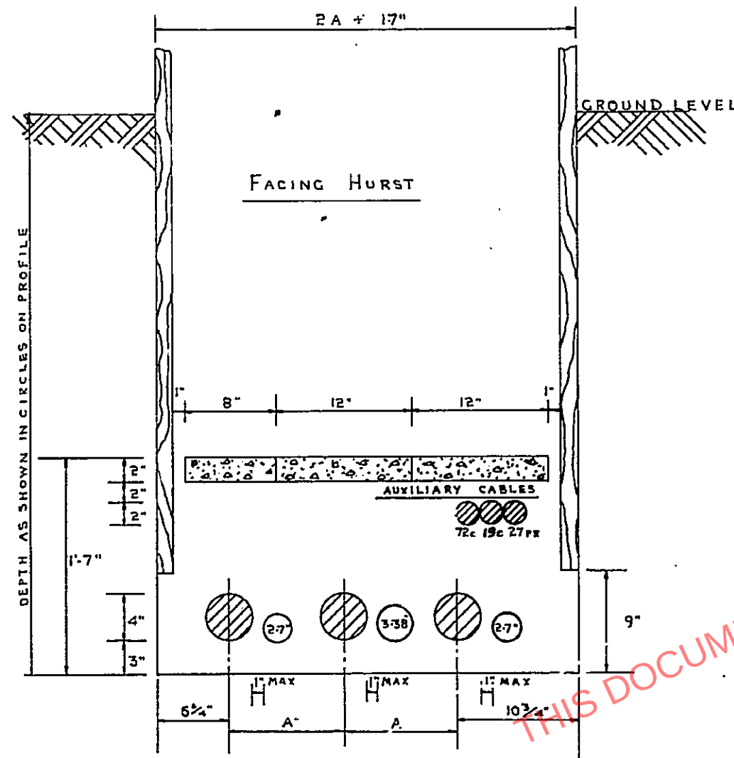
C.S.A. ODD NUMBER CABLE SECTION.
